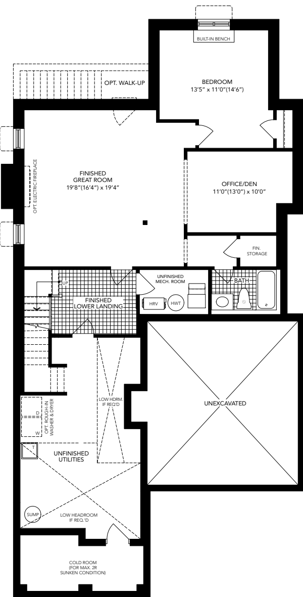
OPT. FINISHED BASEMENT WITH BEDROOM + BATH (ELEV. A)
